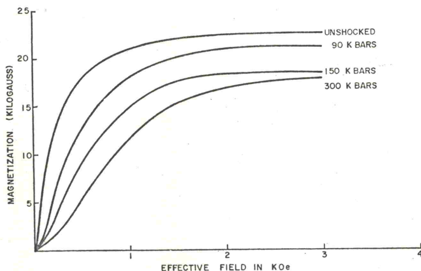
Magnetization curves for iron manganese shock loaded up to 300 kbars.
